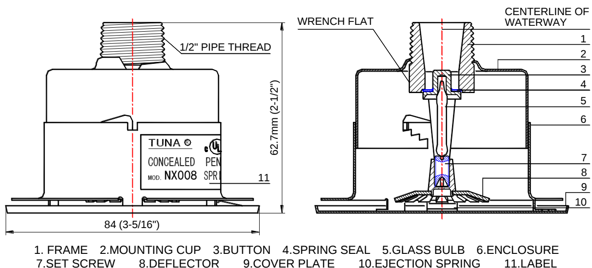
FIGURE A : MODEL NX007/NX008 CONCEALED PENDENT SPRINKLER
